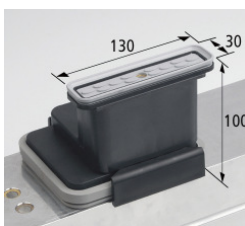
VCBL-K2-130x30x100-L
