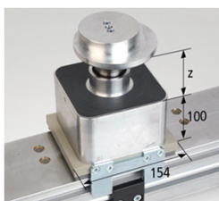
VCMC-K2-154x128x100-10-Fi1
