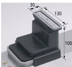
VCBL-K2-130x30x100-Q
