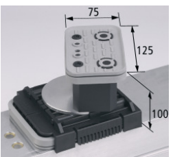
VCBL-K2-125x75x100-D-360
