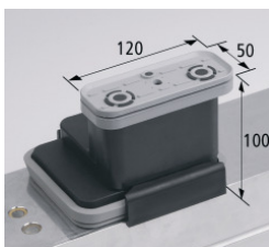
VCBL-K2-120x50x100-L
