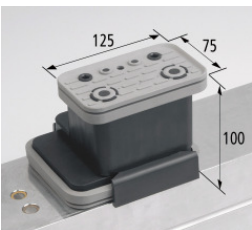
VCBL-K2-125x75x100-L
