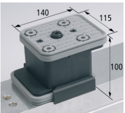
VCBL-K2-140x115x100-AS
